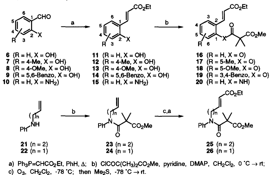
Scheme 1. Synthesis of the Cyclization Substrates
